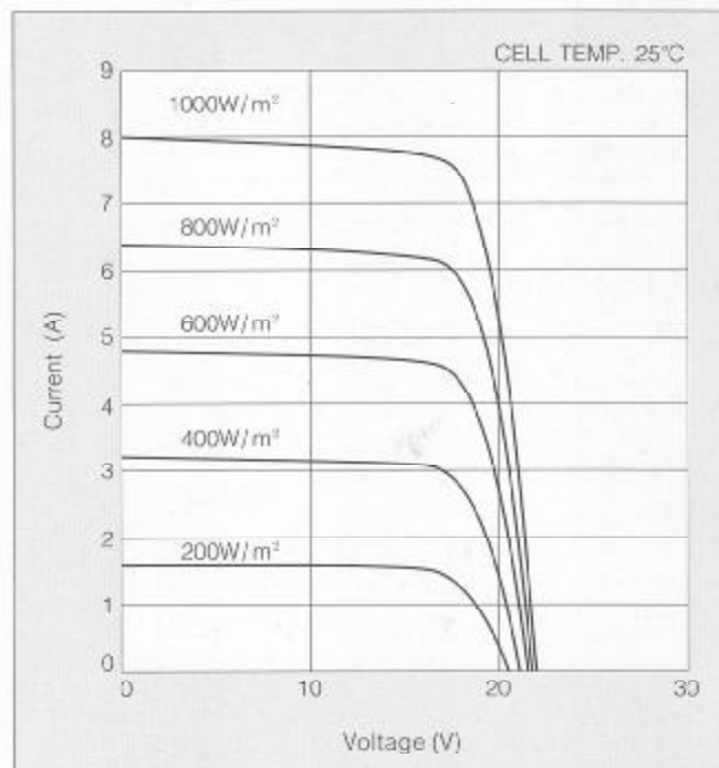
Current-Voltage characteristics of Photovoltaic Module KC130GT at various irradiance levels
