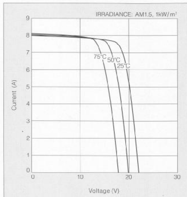
Current-Voltage characteristics of Photovoltaic Module KC130GT at various cell temperatures
