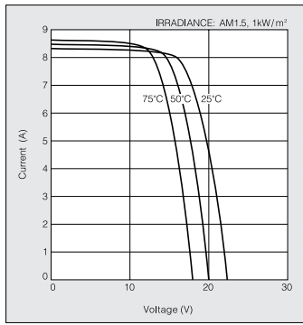
Current-Voltage characteristics of Photovoltaic Module KD135GX-LP at various cell temperatures
