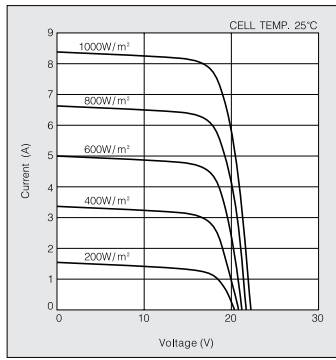
Current-Voltage characteristics of Photovoltaic Module KD135GX-LP at various irradiance levels
